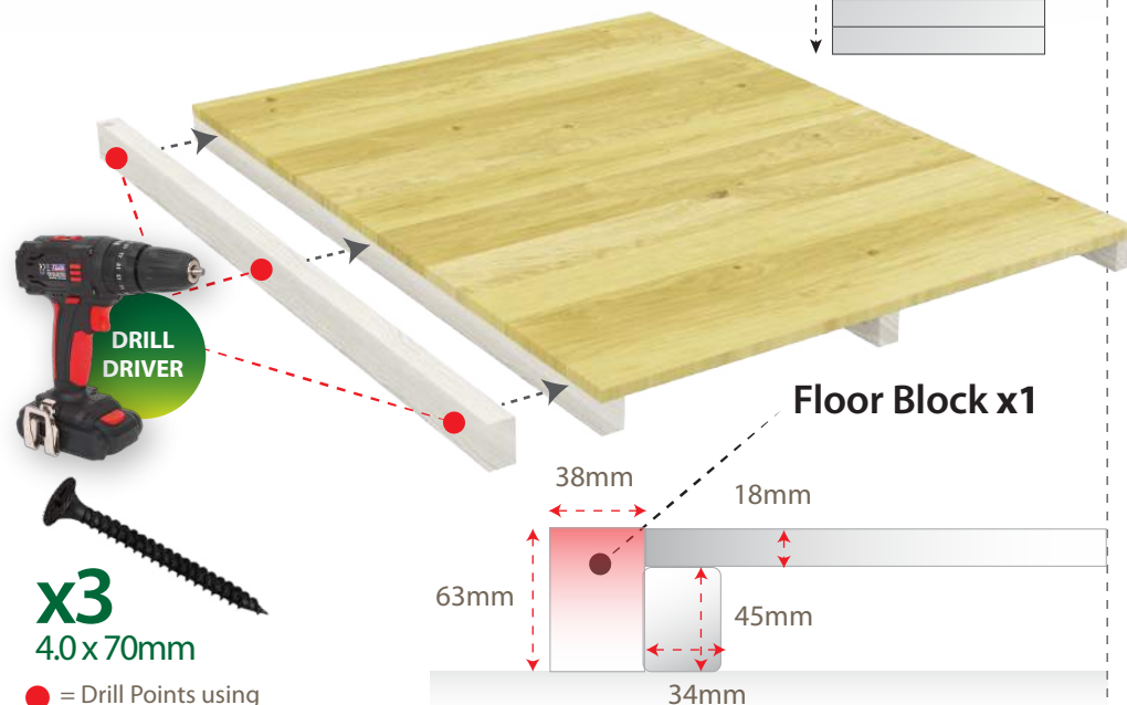
47" Floor Block (63mm x 38mm)
